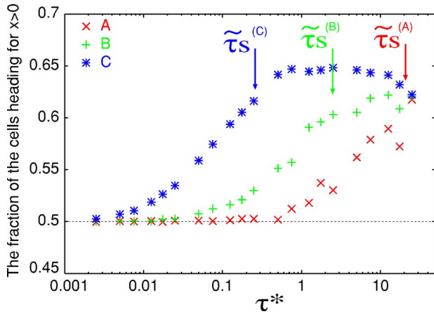
FIG. 5. (Color online) The fraction of cells moving toward the larger x , [i.e., for large S(x) ] at T=100 . The parameters for intracellular dynamics are shown in Table I, in which all conditions are the same as those in Fig. 2. The fraction 0.5 indicates the absence of chemotaxis in short-term behavior.
